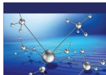
Ghanshyam Purohit Electron impact ionization of atoms and ions
